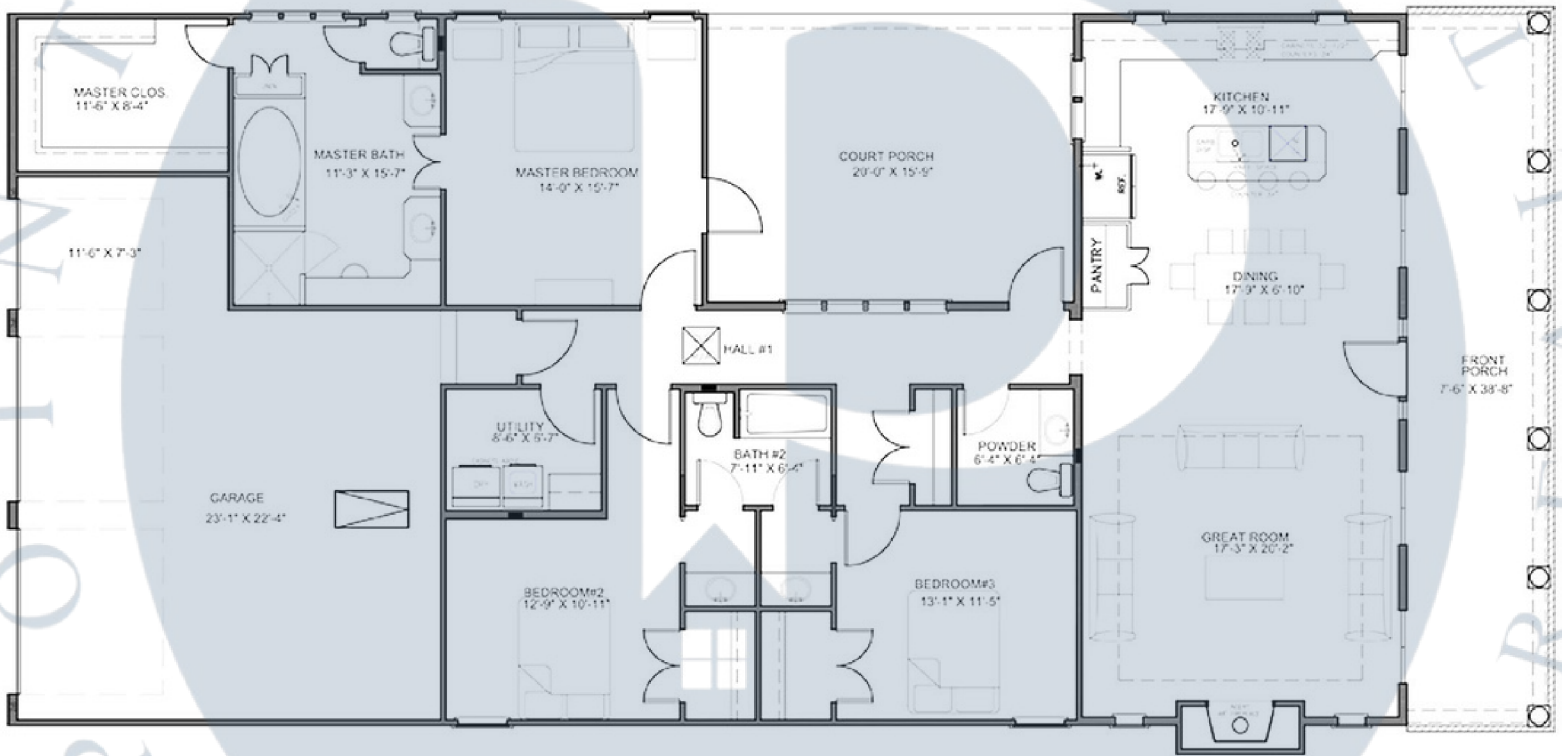
FLOOR PLAN
